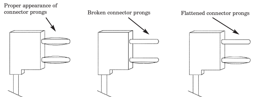
Figure A-4 Inspect Touchpad and Button Connectors
