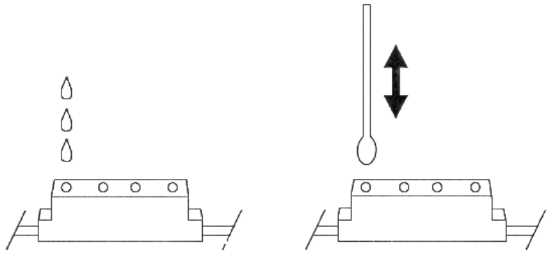
Figure A-3 Clean Cable Connectors as shown
