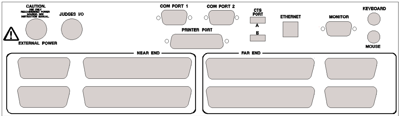
Figure 2-H System 6 I/O Panel
