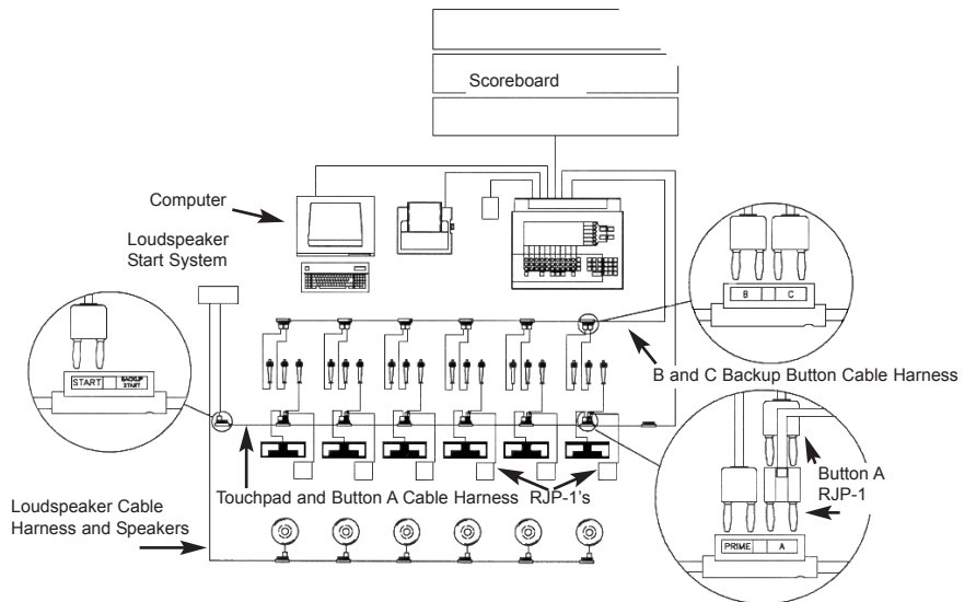
Figure 2-G Full System
