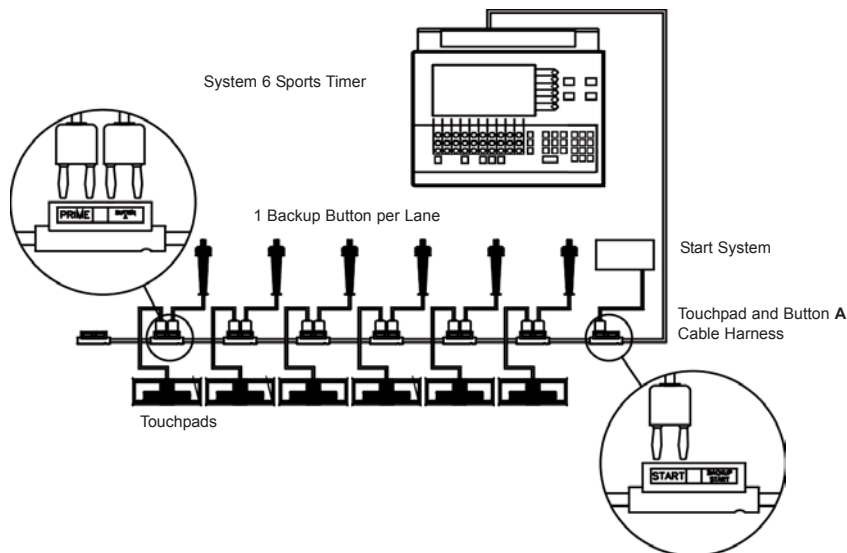
Figure 2-E Touchpad Finish/1-Button Backup
